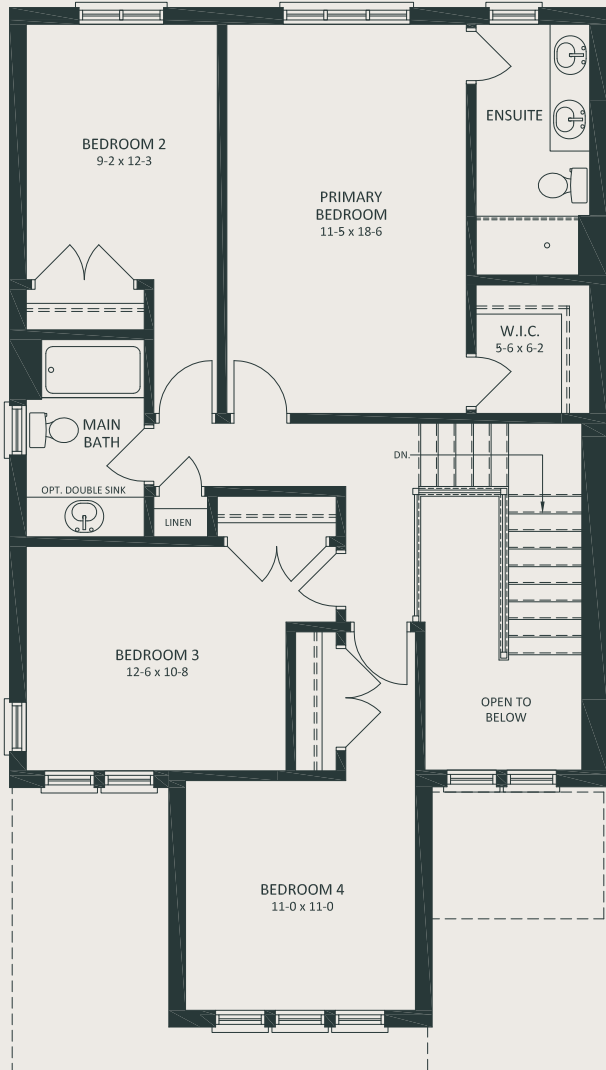
SECOND FLOOR
