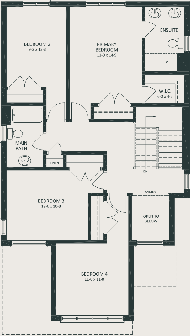
SECOND FLOOR
